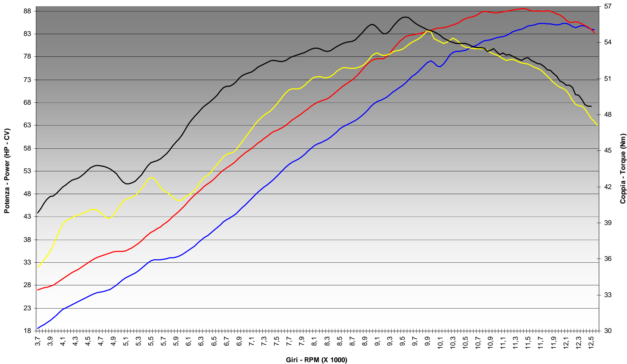
Max Power and Torque Dynochart
